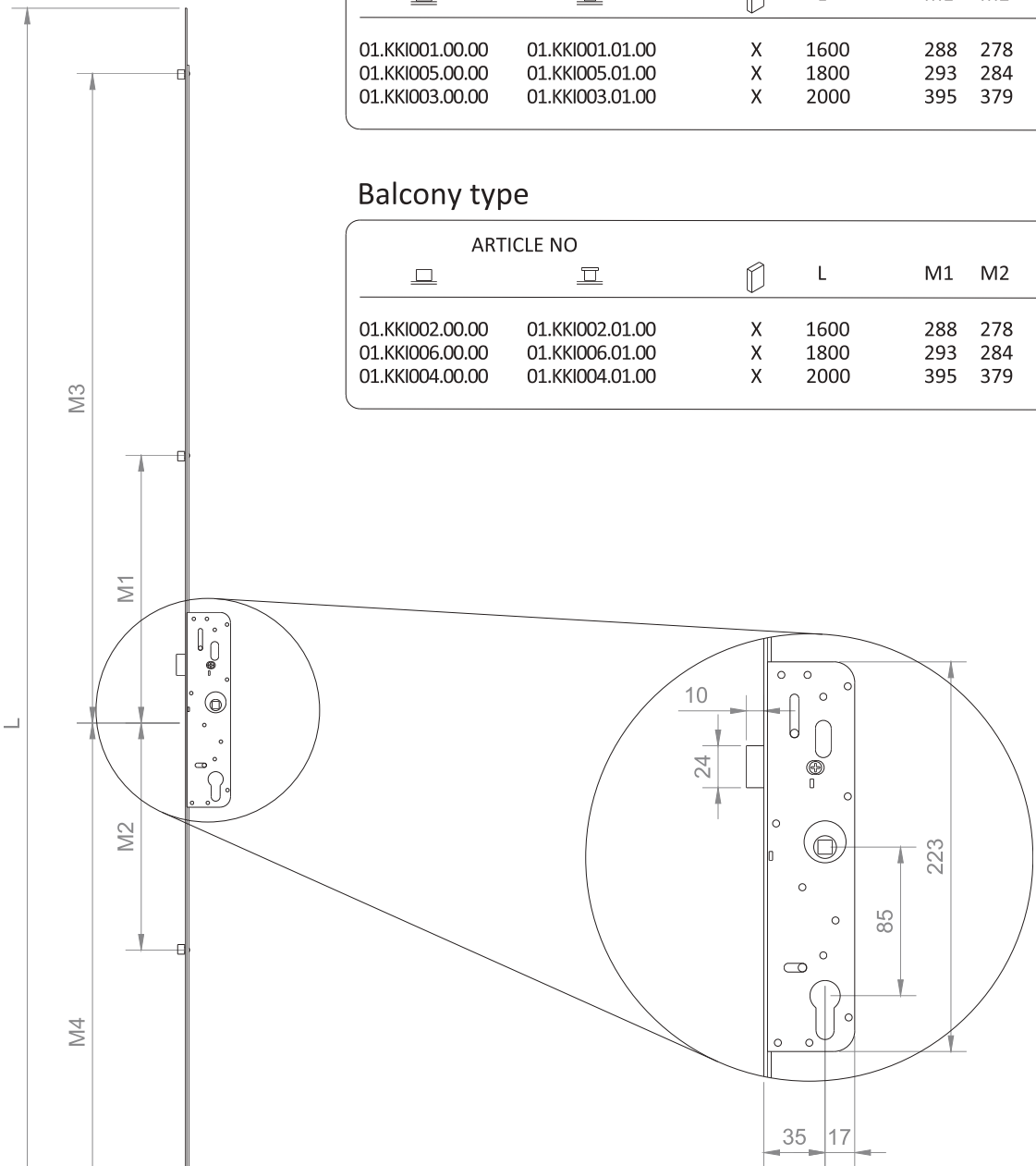
Standard profile cylinder type
