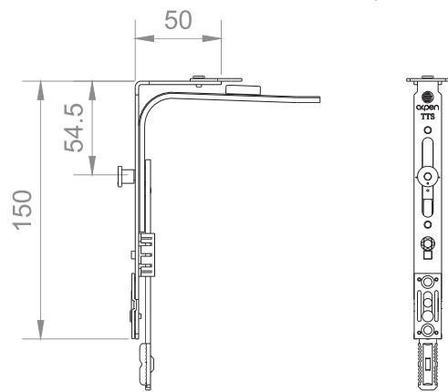
Small Corner Transmission 150x50, 1 SeML
