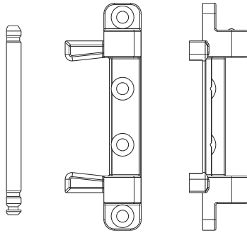
Stay arm bearing with anchorage 100 kg
