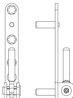
Corner bearing 130 kg
