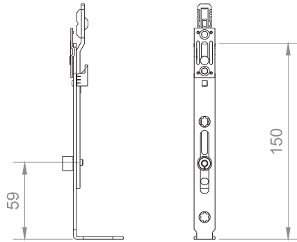
Bottom Extension 180°
