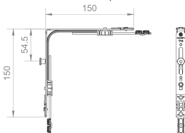
Corner Transmission 150x150, 1 SeML
