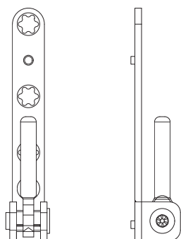
Corner bearing 100 kg
