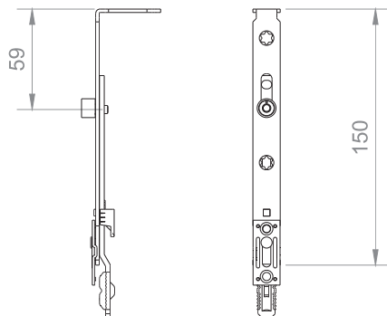
Bottom Extension 90°
