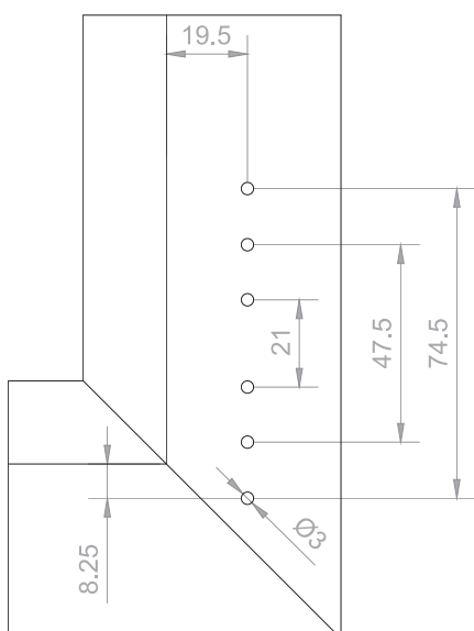
Drilling for corner bearing 100 kg
