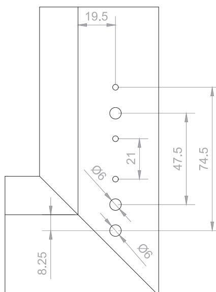
Drilling for corner bearing 130 kg
