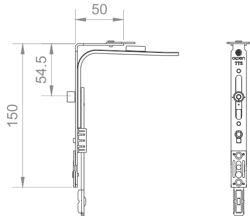
Small Corner Transmission 150x50, 1 ML
