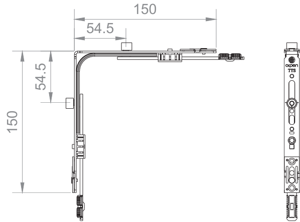
Corner Transmission 150x150, 2 ML
