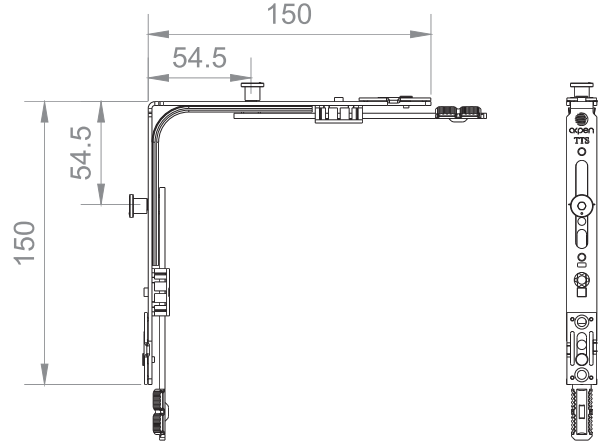
Corner Transmission 150x150, 2 SeML
