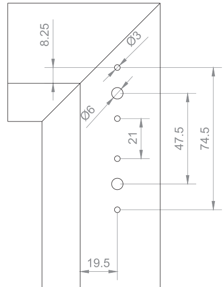
Drilling for stay arm bearing 130 kg
