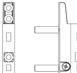
Drill-in corner hinge 130 kg
