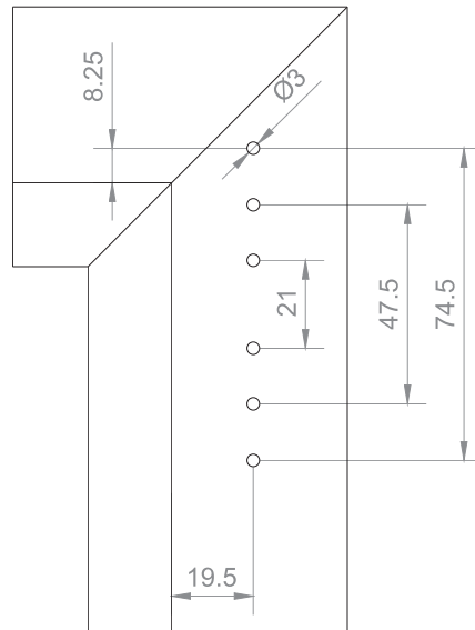
Drilling for stay arm bearing 100 kg
