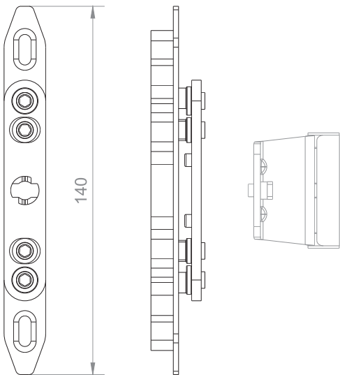
3D Adjustable Middle hinge
