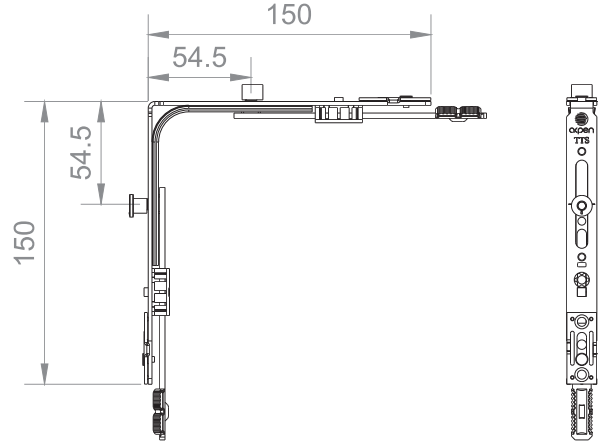
Corner Transmission 150x150, 1 ML, 1 SeML
