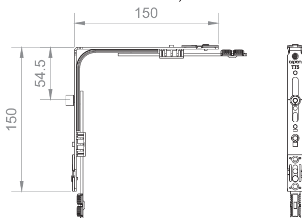
Corner Transmission 150x150, 1 ML
